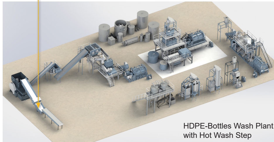
HDPE-Bottles Wash Plant
